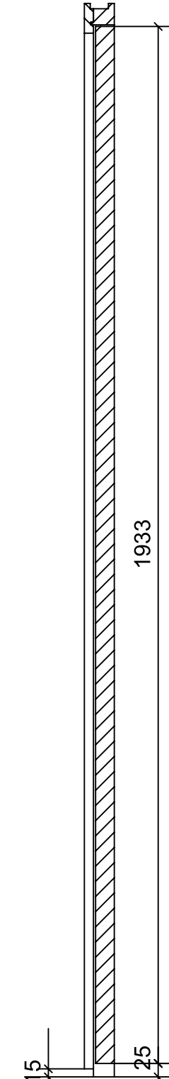
SECTION C-C
