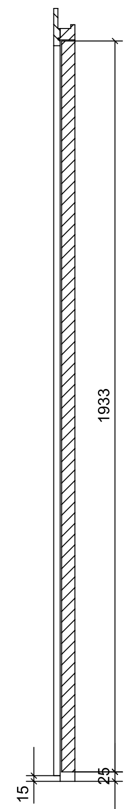
SECTION C-C
