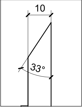
DETAIL K SCALE 1:1
