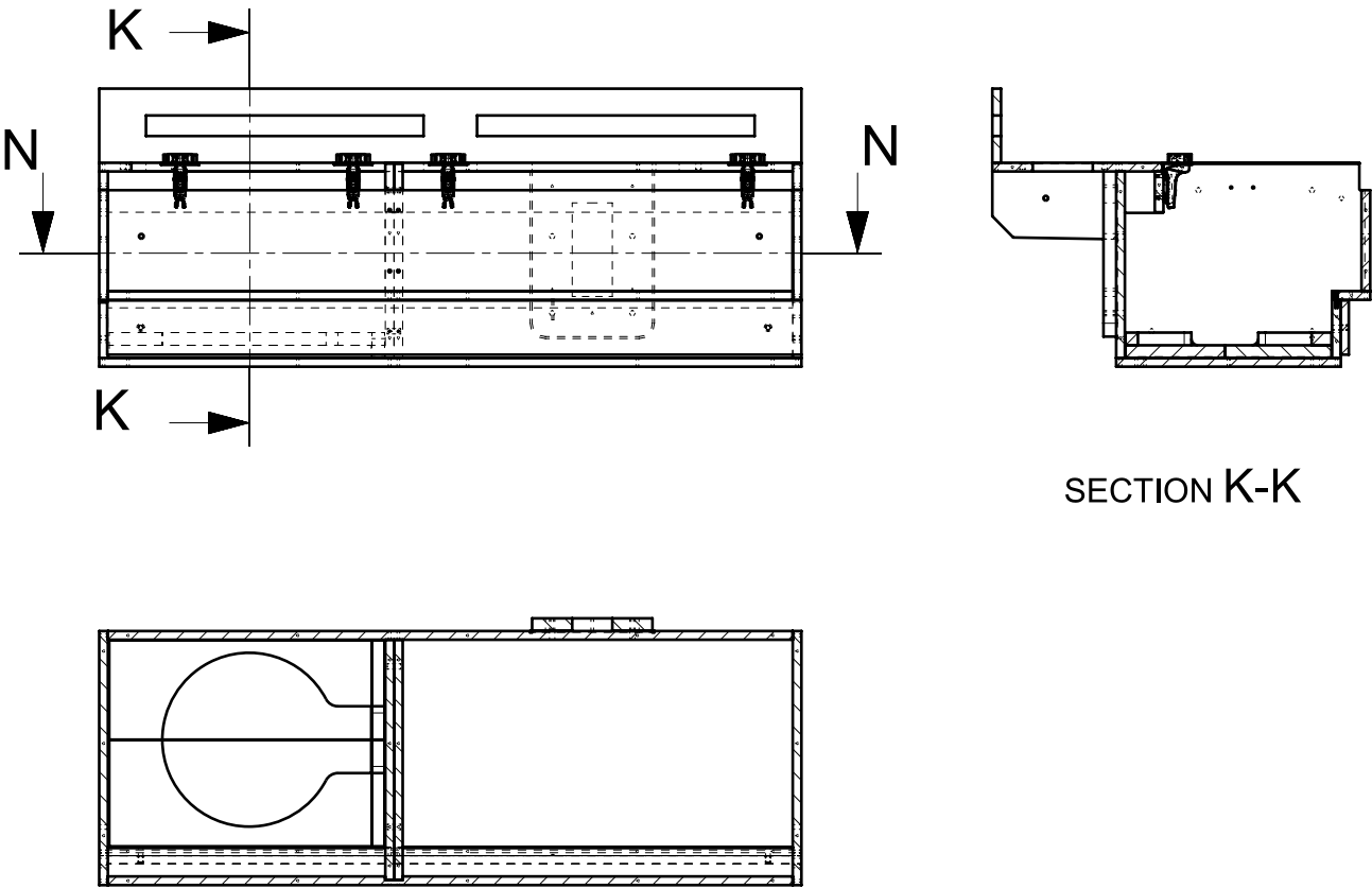
SECTION N-N
