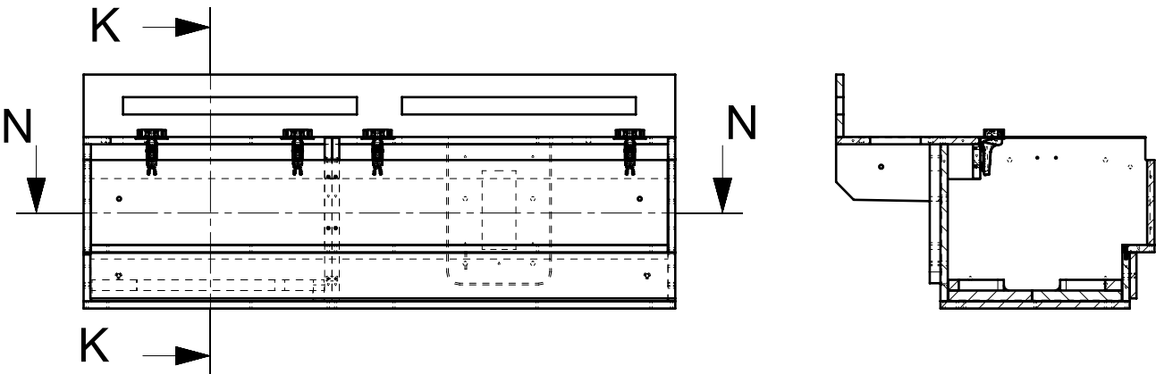
SECTION K-K
