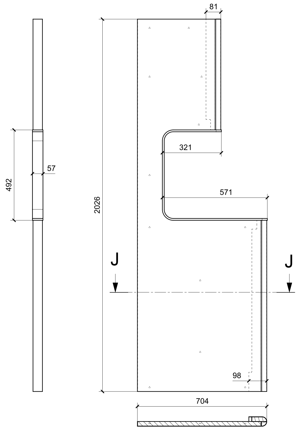
SECTION J-J
