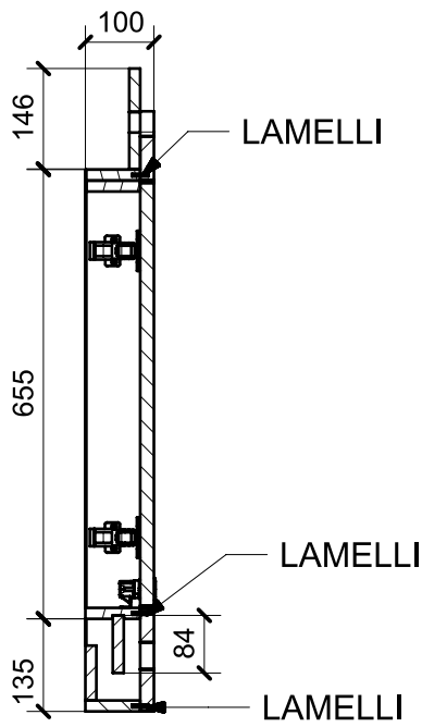
SECTION E-E
