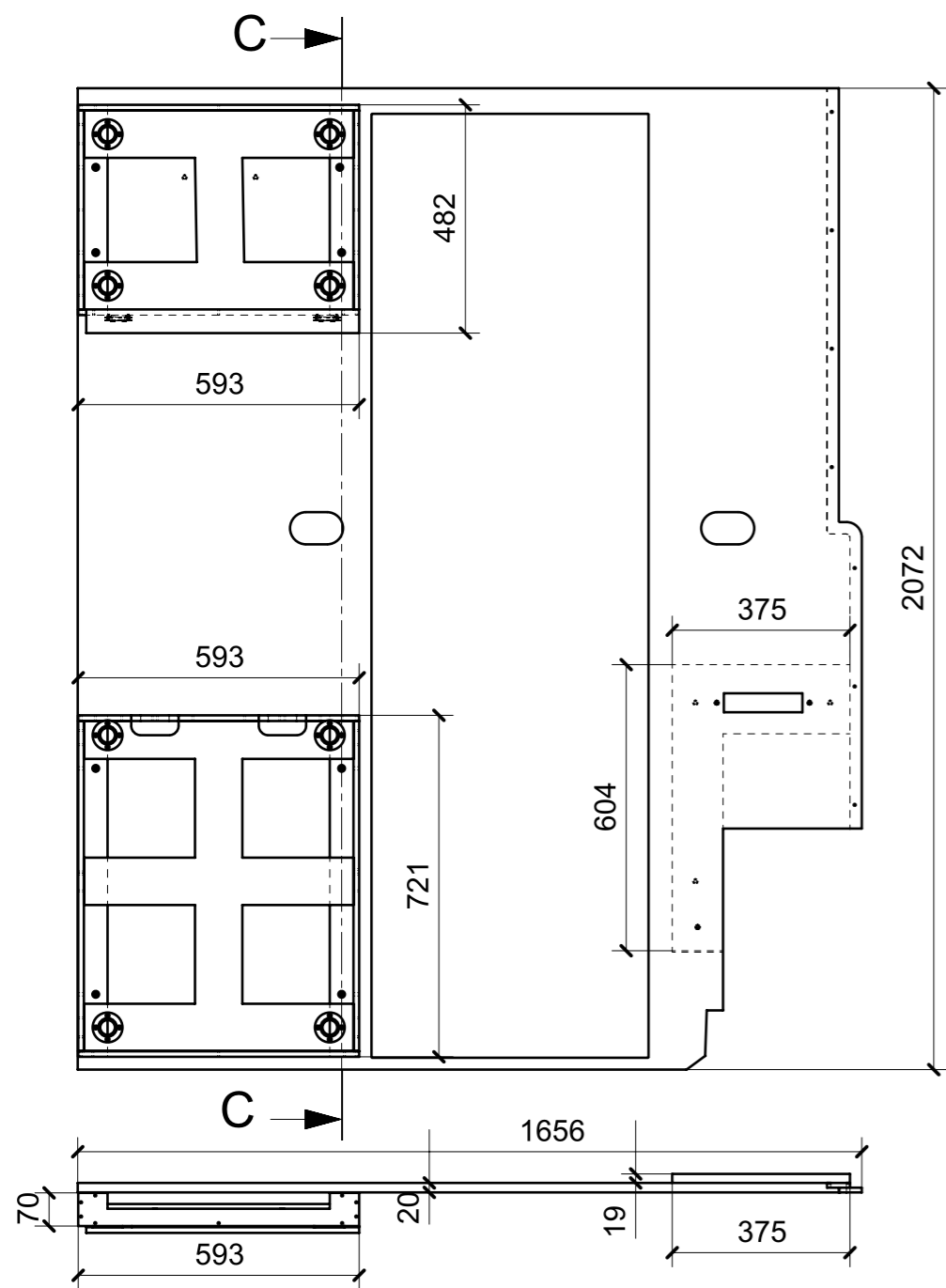
SECTION C-C
