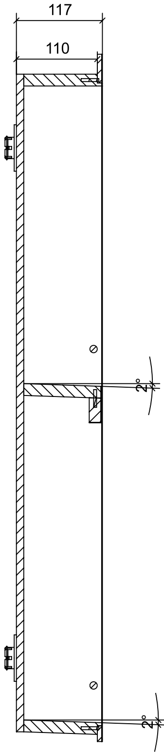
SECTION J-J
