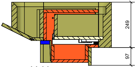
SECTION H-H
