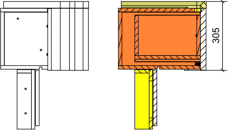
SECTION K-K
