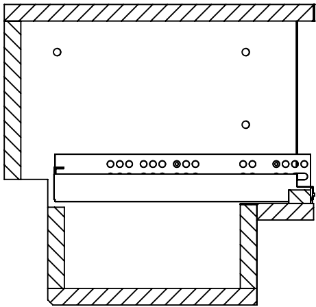
SECTION F-F
