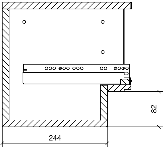
SECTION S-S
