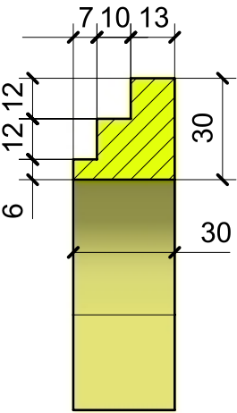
SECTION AB-AB
