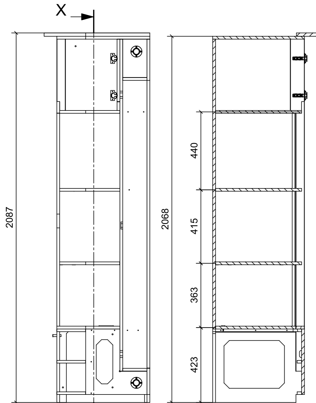
SECTION X-X
