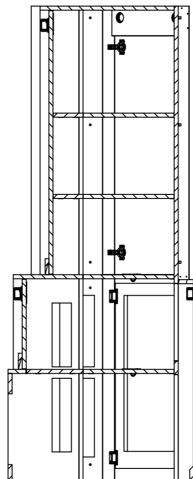
SECTION Z-Z
