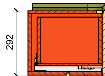
SECTION N-N
