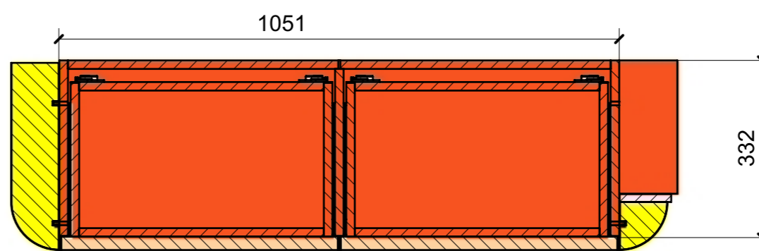
SECTION N-N
