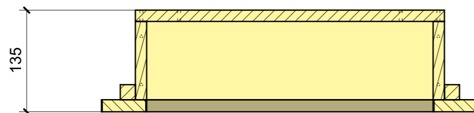
SECTION C-C
