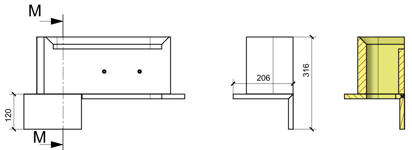
SECTION M-M
