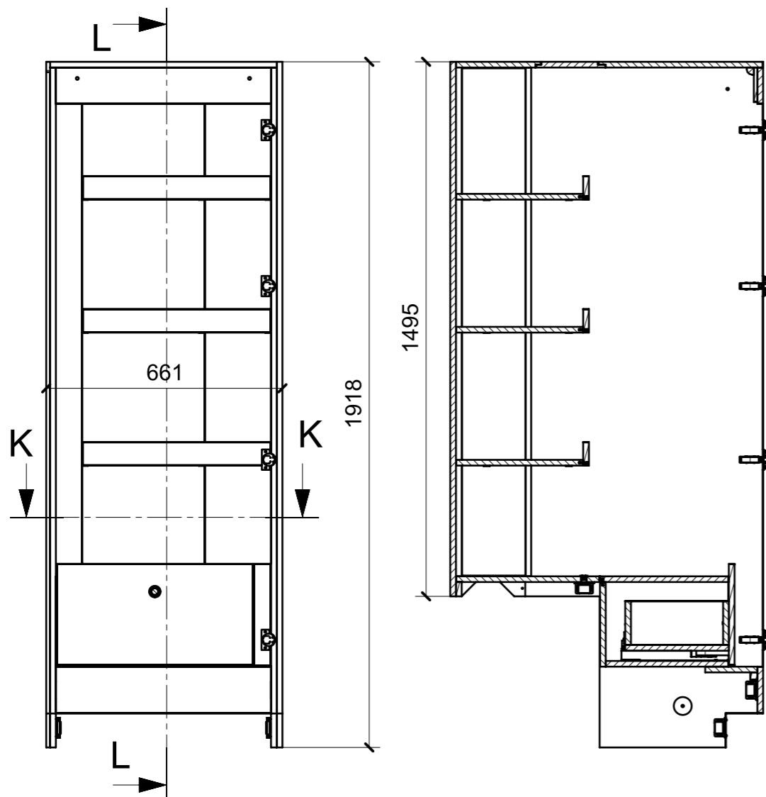
SECTION L-L
