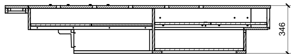
SECTION L-L
