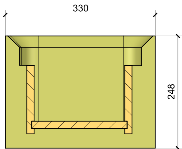
SECTION L-L
