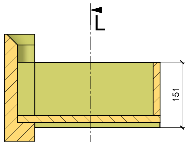
SECTION K-K
