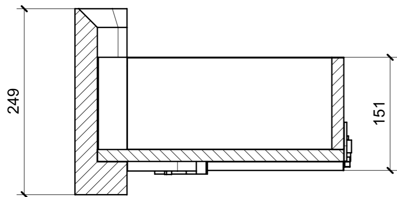
SECTION R-R
