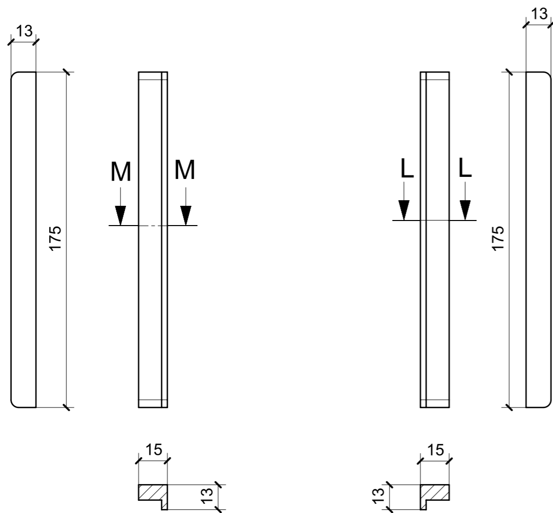
SECTION M-M
