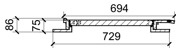
SECTION P-P
