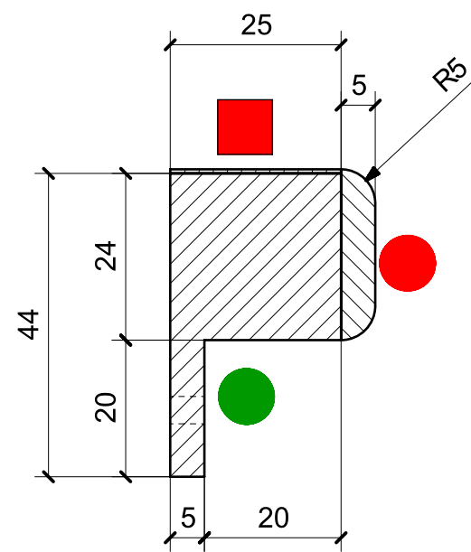
SECTION E-E SCALE 1:1
