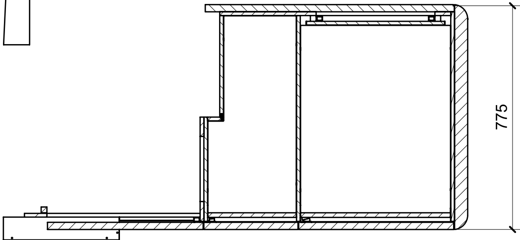
SECTION N-N
