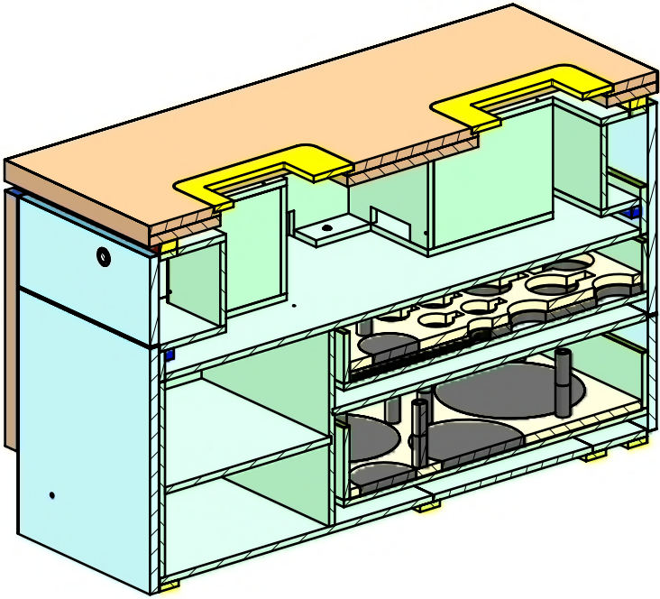
SECTION X-X
