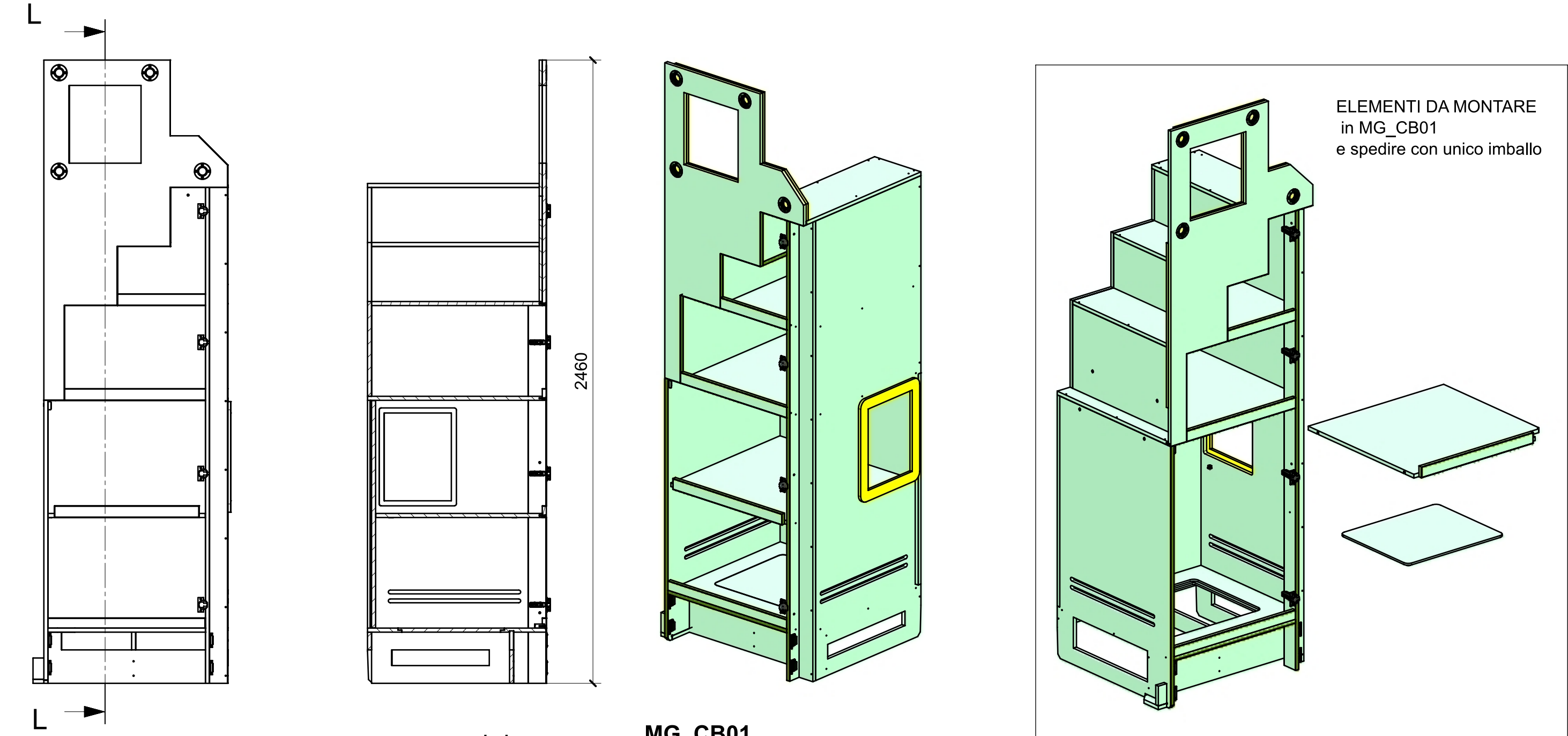
SECTION L-L
