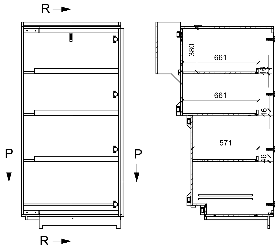
SECTION R-R
