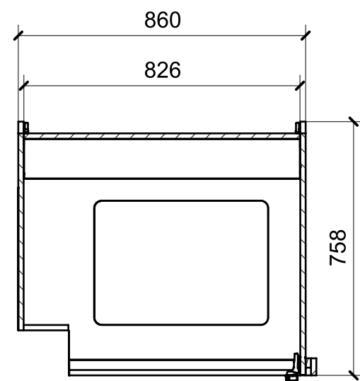
SECTION P-P
