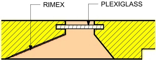
DETAIL V
