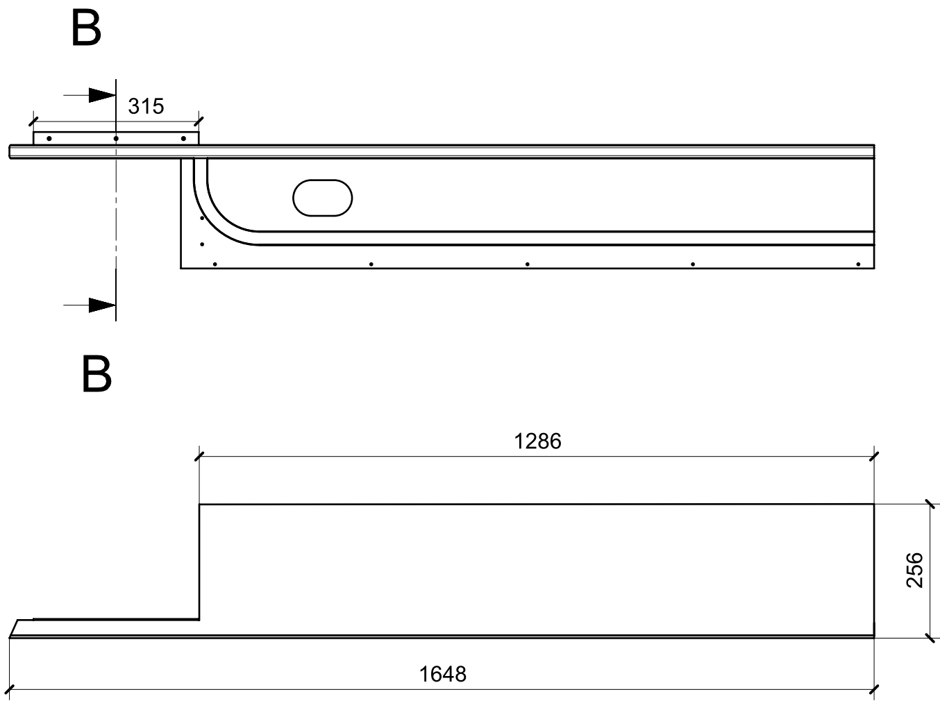
SECTION B-B
