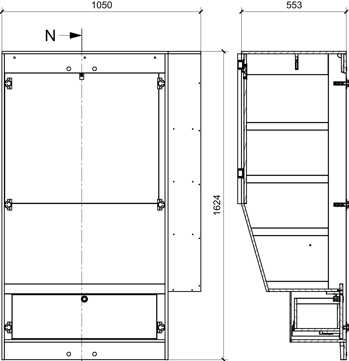
SECTION N-N
