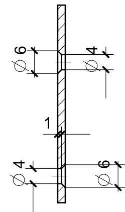
SECTION G-G
