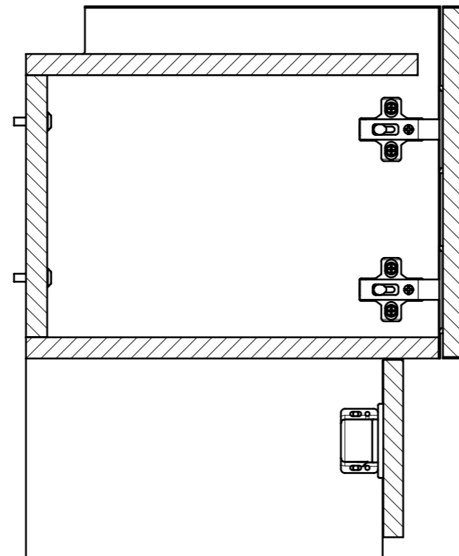
SECTION F-F
